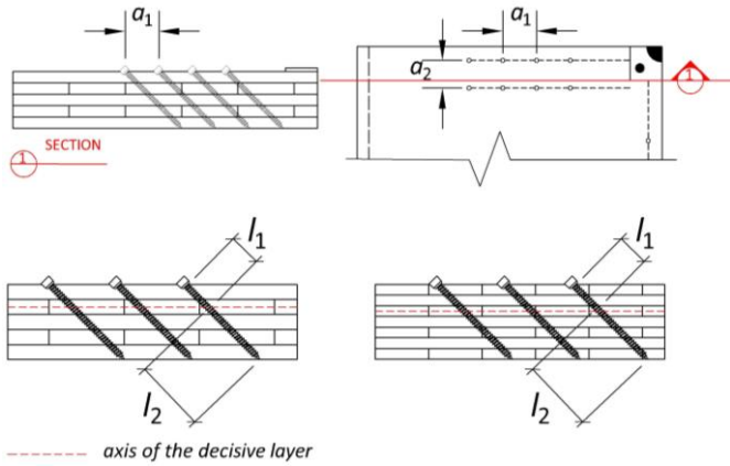
Figure 1. Geometric parameters of Mestek and Dietsch model.
