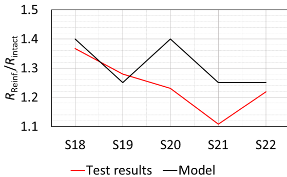
Figure 7. Punching shear test results vs. analytical model.
