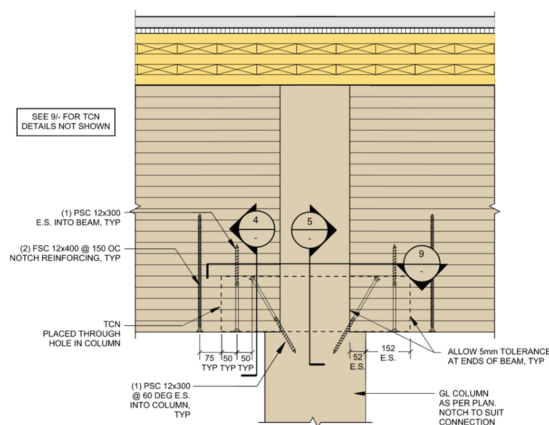
Figure 4 – TCN Assembly Detail
