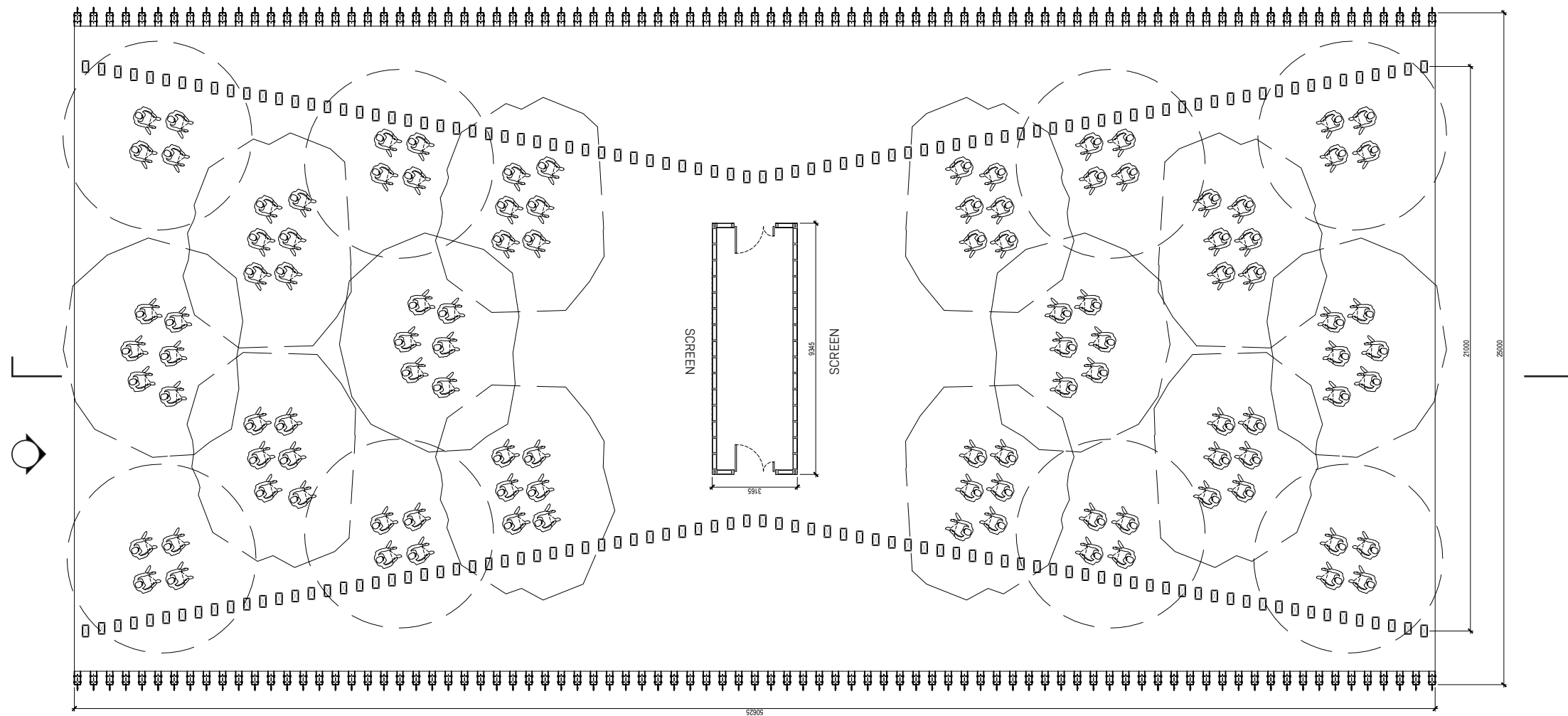
PLAN 1:200
