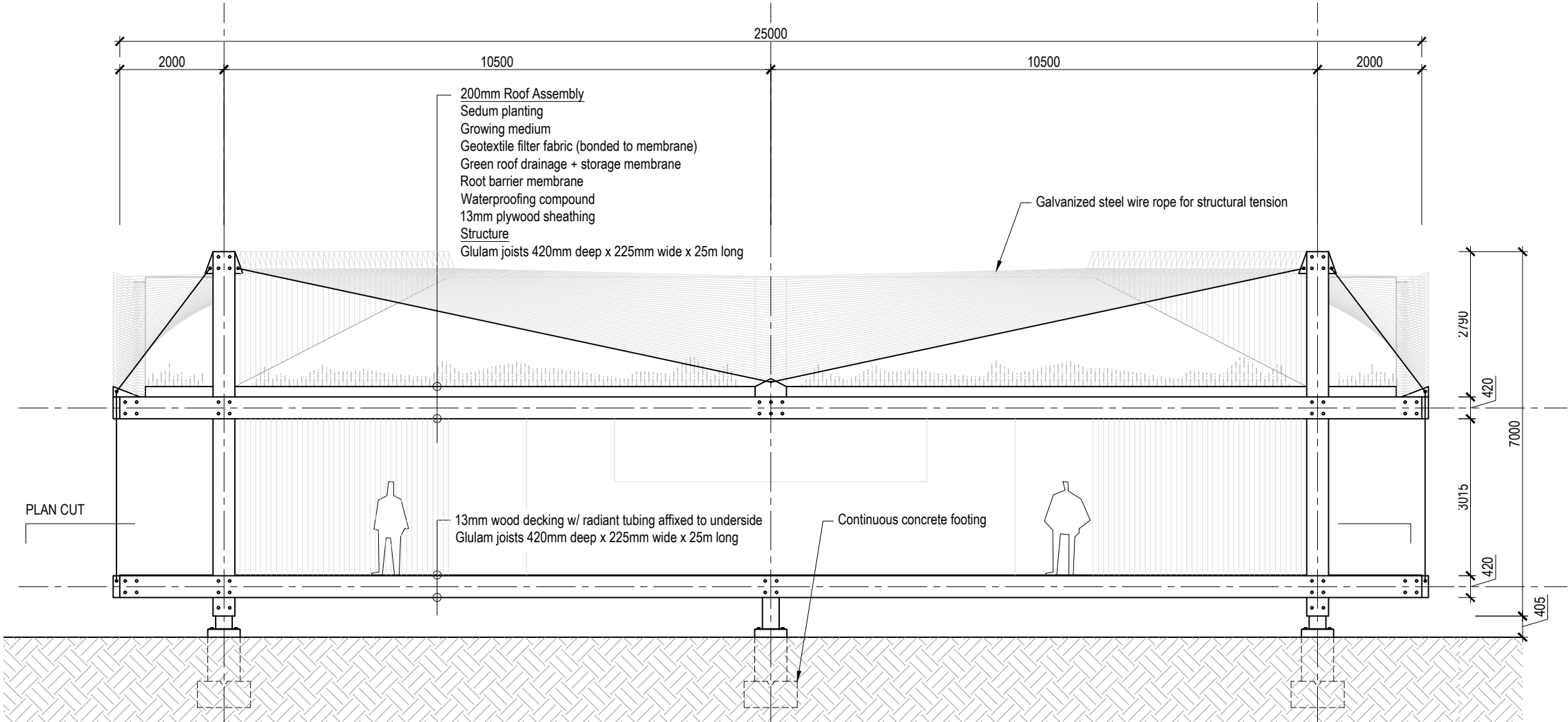
ELEVATION AT ENTRANCE 1:100
