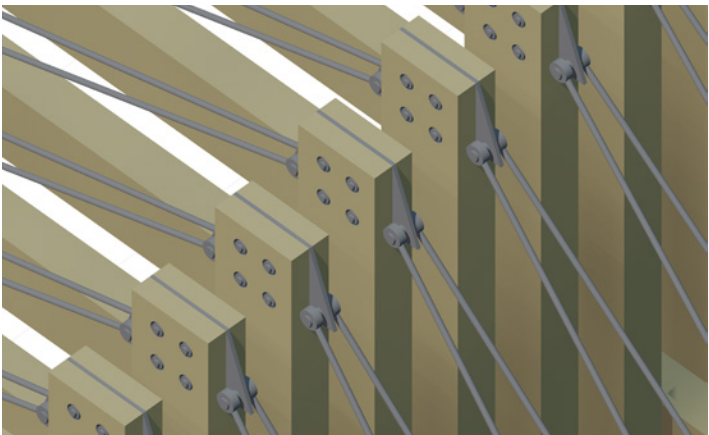
TOP-OF-COLUMN CABLE CONNECTION Top-down isometric view
