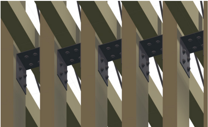
BEAM-TO-COLUMN CONNECTION Bottom-up isometric view
