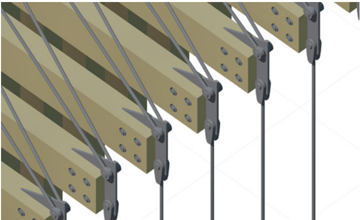
END-OF-BEAM CABLE CONNECTION Top-down isometric view
